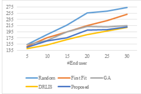
(a) CPU balancing in low load
