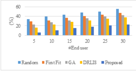
(a) Critical deadline violation in heavy load
