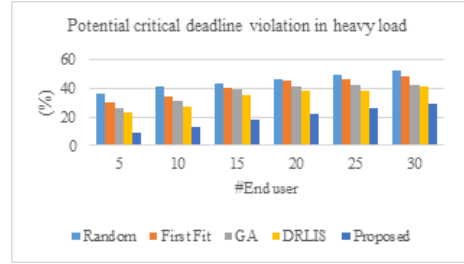
(b) Potential critical deadline violation in heavy load
